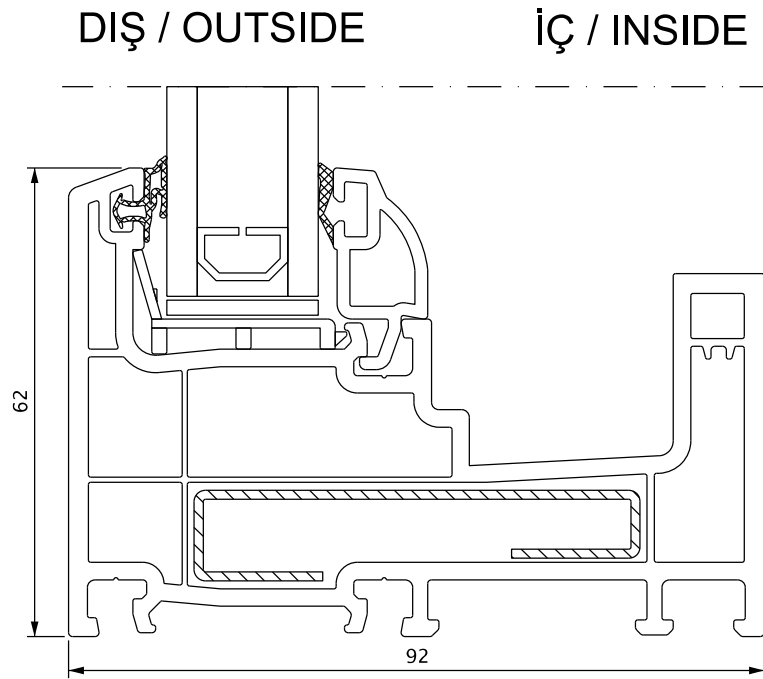
SBT.BLM. SÜRME KASA FIXED SLIDING FRAME
